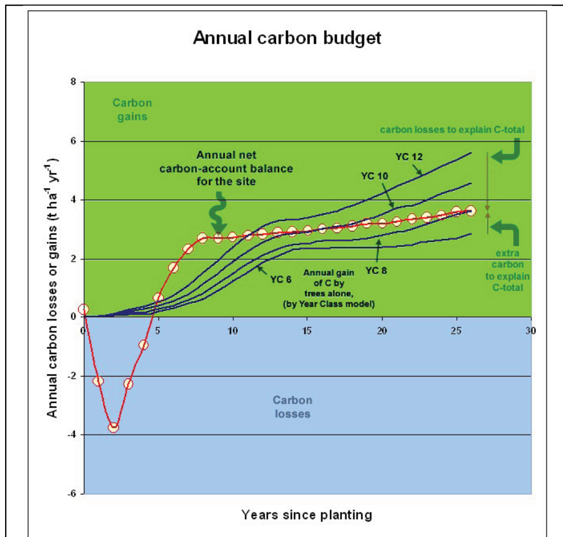
Figure 45. Carbon balance model constructed for 26 years of forestry on peat by Hargreaves et al. (2003). The net accumulated carbon for the afforested peatland site is shown by the red line. Dark blue lines represent modelled carbon-accumulation curves for the timber of conifer forests growing at differing Yield Classes. The pale blue lower zone of the graph is when the net accumulation of carbon within the site is negative ( i.e. lost to the atmosphere), the green upper zone of the graph is where the net carbon accumulation of carbon on the site is positive ( i.e. the site gains carbon). Where the red line lies below a modelled Yield Class line, the site is losing carbon through oxidation even though the trees may be gaining carbon, the difference between the lines showing how much carbon is lost. Where the red line is above a modelled Yield Class line, the site is gaining carbon faster than can be explained by the growing trees, and must therefore still be forming peat in remnant areas of vegetation.
