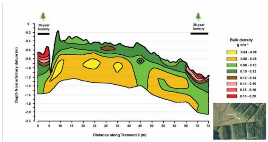
Figure 13. Bulk density profile along Transect 2, Bad á Cheo, Caithness.
