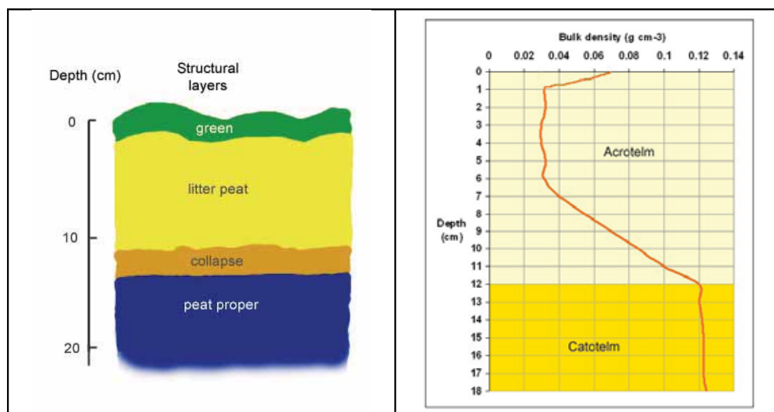
Figure 6. Layering and bulk density in the surface layers of a bog (after Clymo, 1992).
