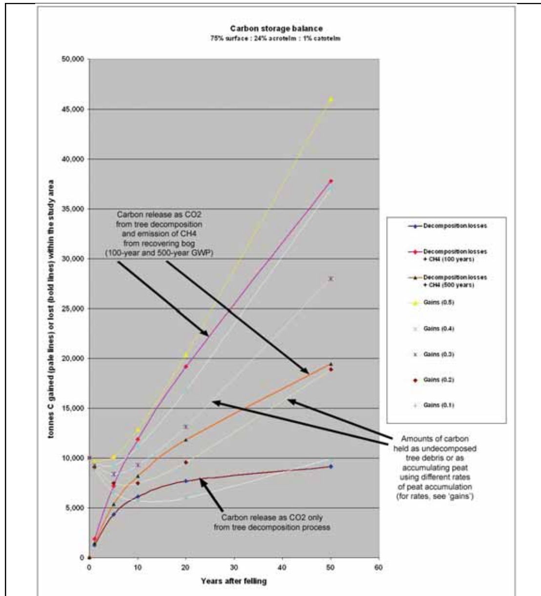
Figure 47. Carbon accumulation rates and carbon losses for 15-year felled forestry
