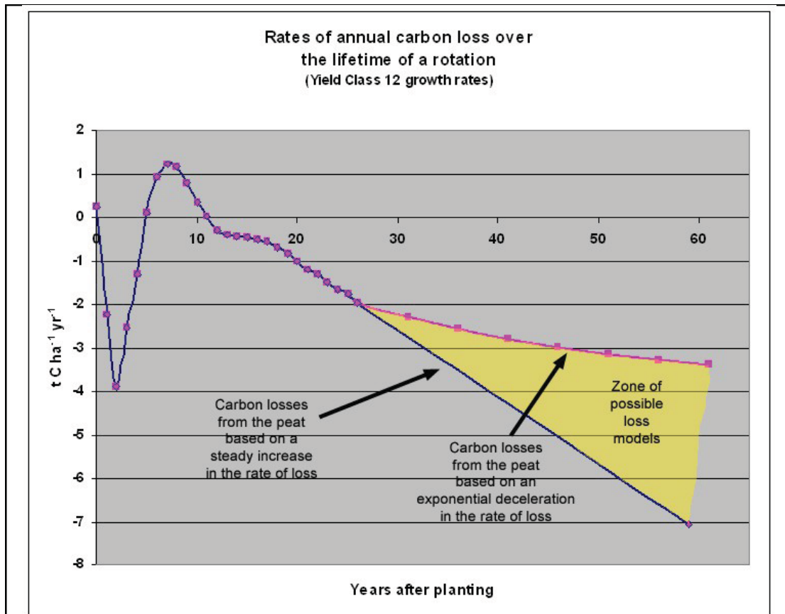
Figure 46. Carbon balance over 60 years for Yield Class 12 trees planted on peat.
