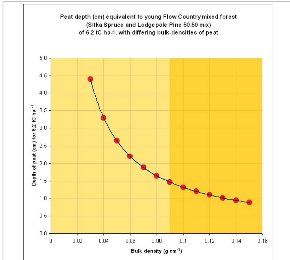
Figure 48. Thickness-equivalence of a Sphagnum carpet vs forest carbon biomass for a 15-year mixed forest.
